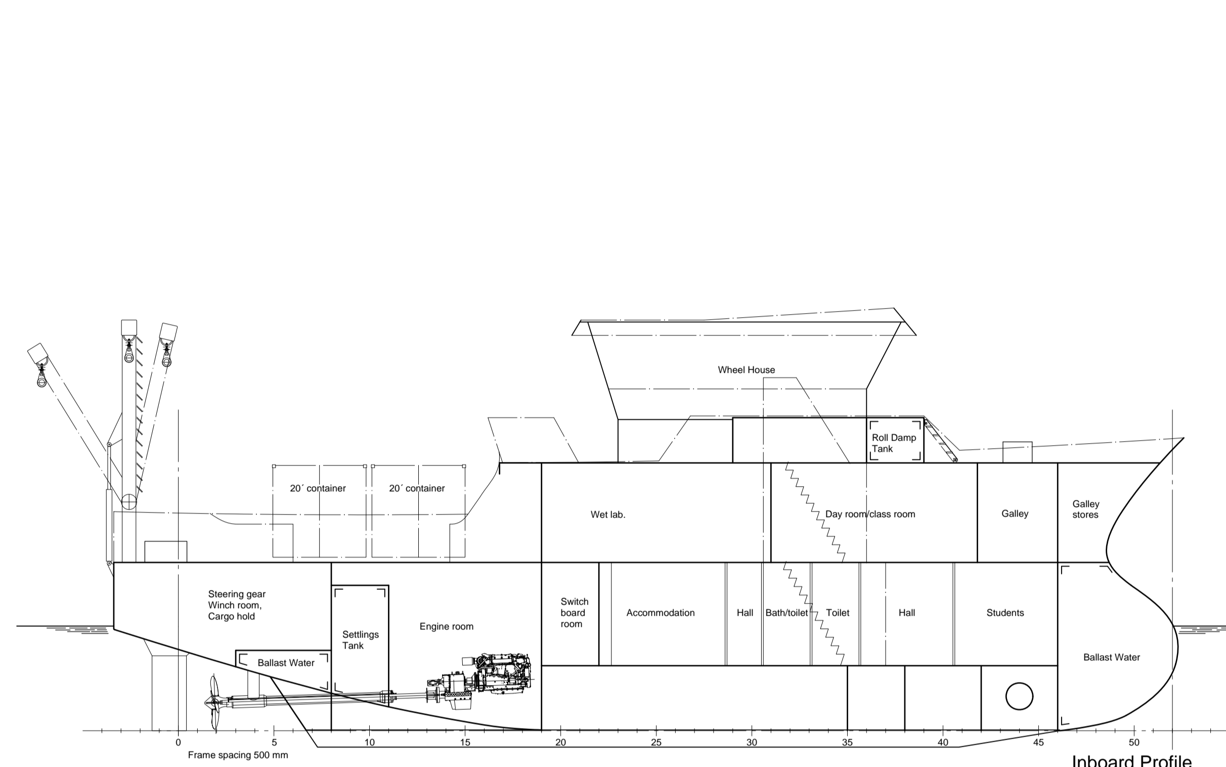
Inboard Profile
